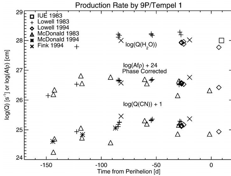
Figure 2. Production rates for OH, CN and dust, from Lowell Observatory narrowband photometry, IUE measurements and IDS spectra from McDonald Observatory. The middle set of data points shows the phase-corrected values of Afp from the narrowband photometry as a reference. The lower points show the variation of production of CN from both narrowband photometry and spectrophotometry. The CN and the dust curves both show excellent agreement between the 1983 and 1994 apparitions. The upper points show the production rates of H_2O deduced from narrowband photometry of OH at both apparitions, from IUE spectra of OH (reduced with the same parameters) in 1983 and from ground-based spectrophotometry of O(1D) in 1994. Unlike the other species (including those not shown here), there may be a factor of two reduction in water production from 1983 to 1994.
