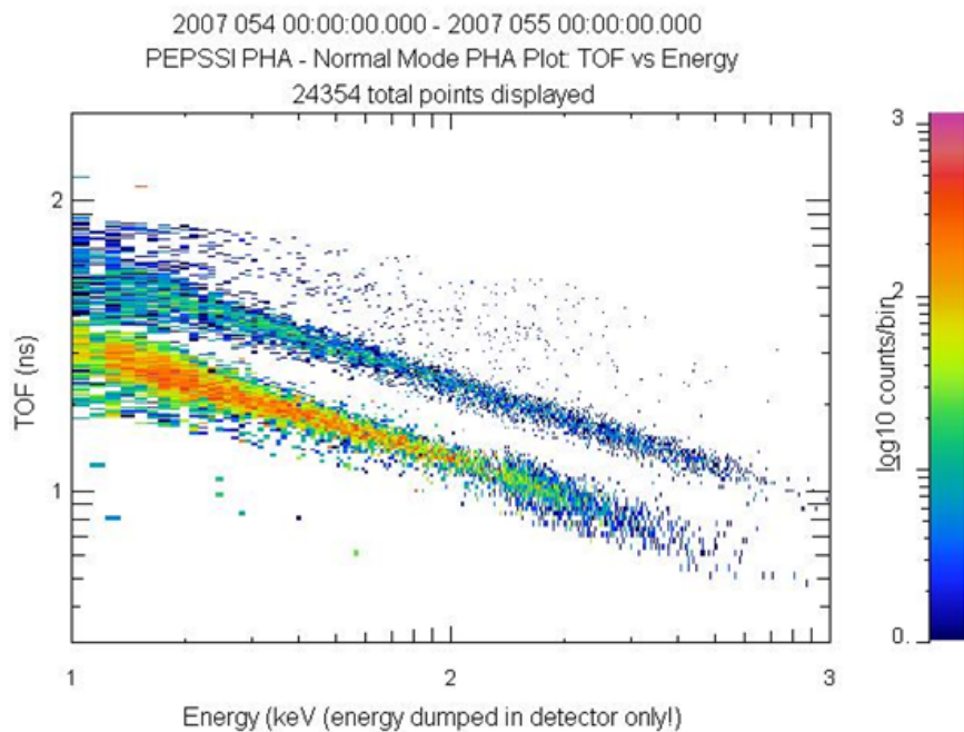
Figure 11-9: 2D PHA Histogram with Rate-Weighting applied.
