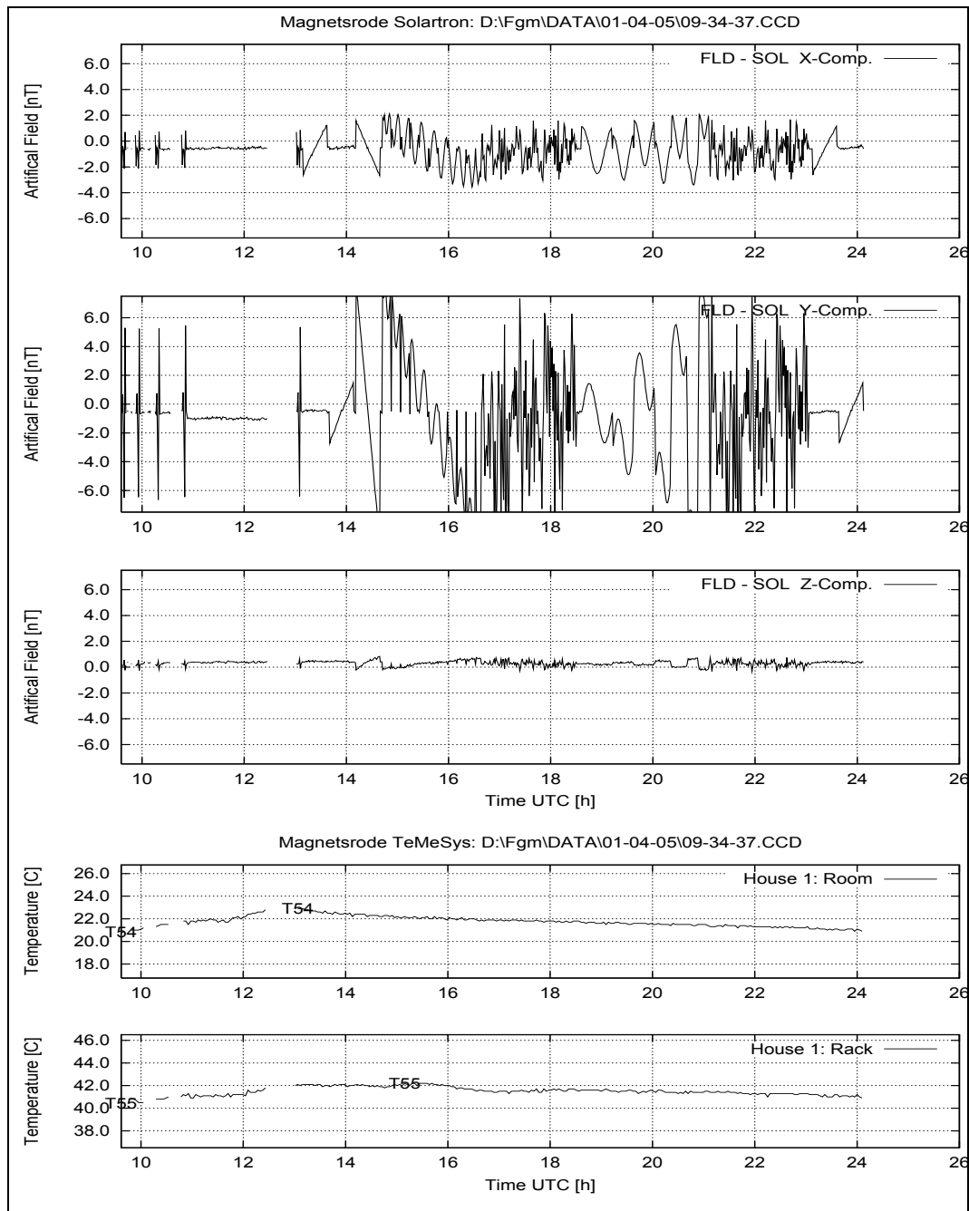
Figure 46: April 5, 2001: System Performance: FLD – SOL; Temperatures at House 1.
