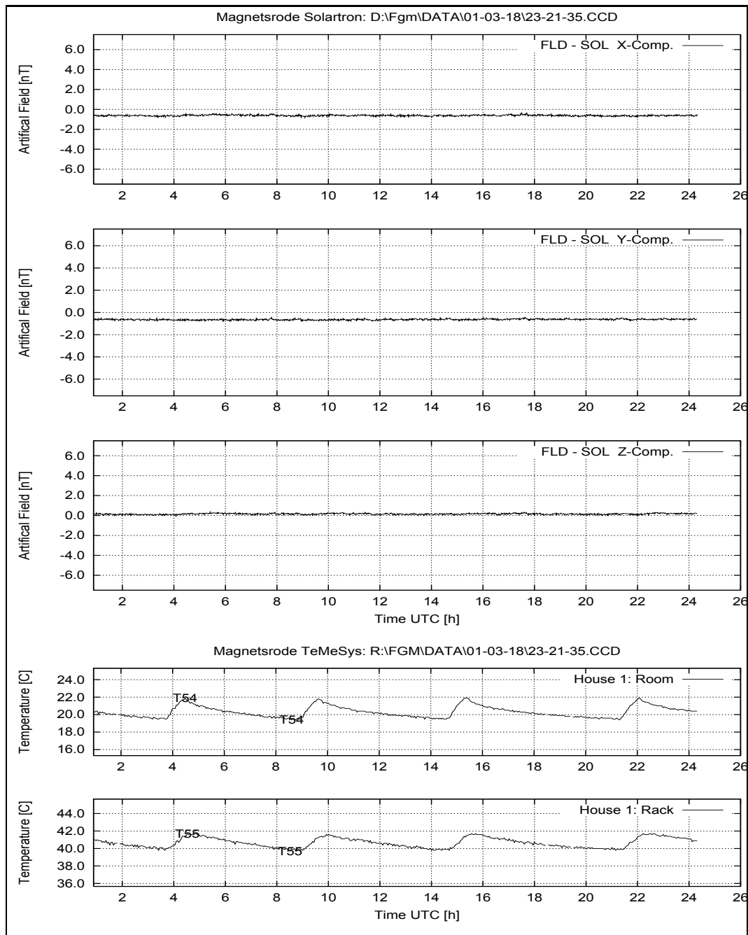
Figure 217: March 18, 2001: System Performance: FLD – SOL; Temperatures at House 1.
