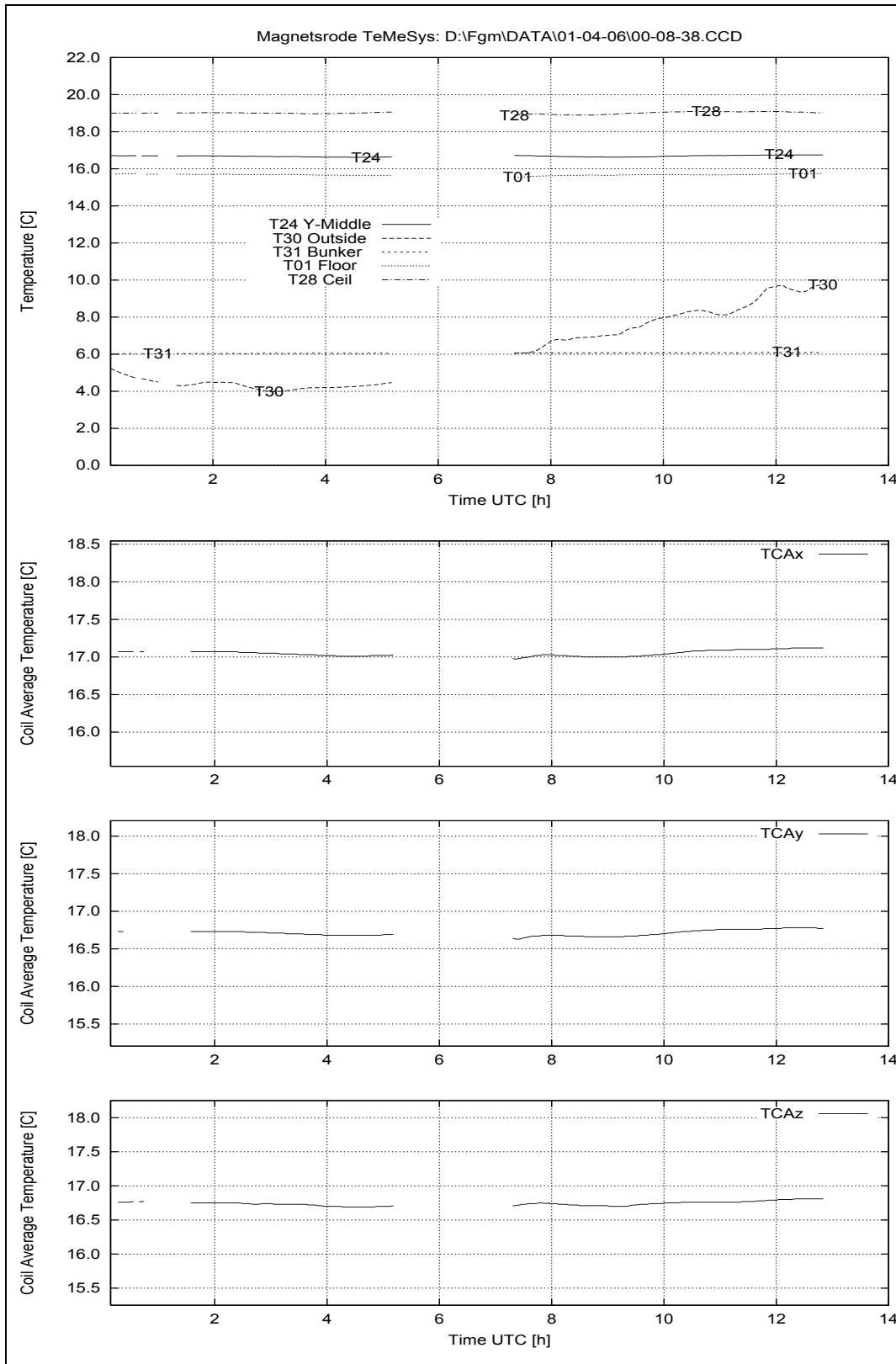
Figure 51: April 6, 2001: Temperatures House 2.
