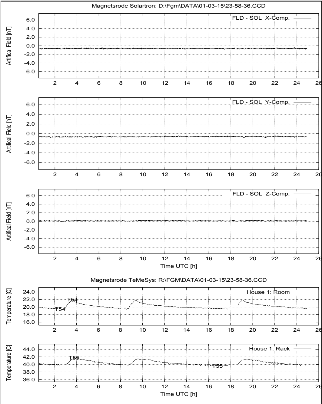
Figure 205: March 15, 2001: System Performance: FLD – SOL; Temperatures at House 1.
