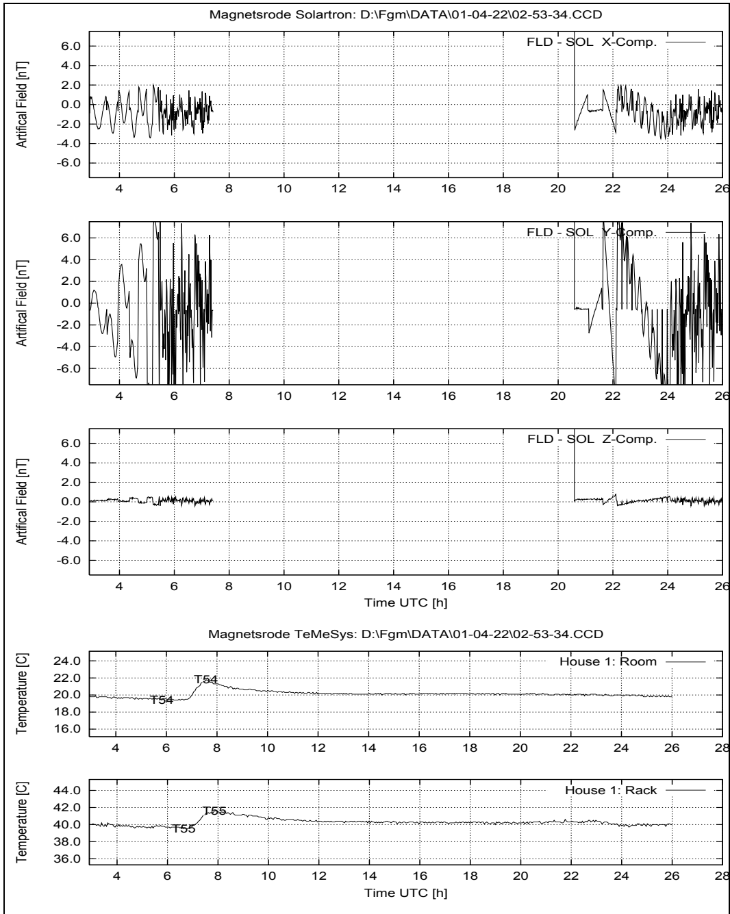
Figure 66: April 22, 2001: System Performance: FLD – SOL; Temperatures at House 1.
