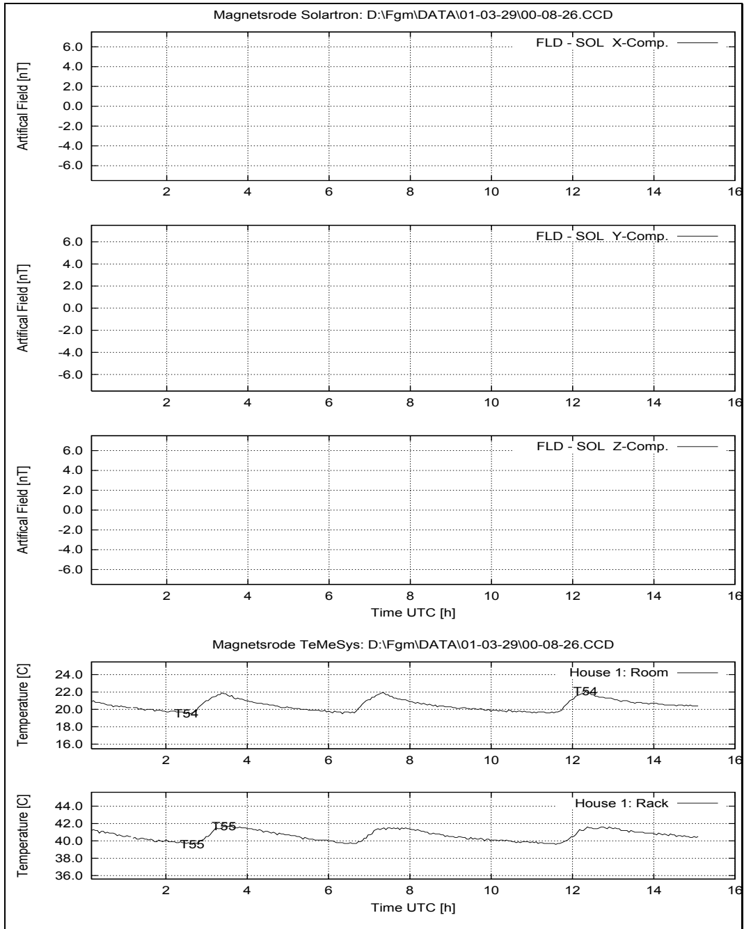
Figure 42: March 29, 2001: System Performance: FLD – SOL; Temperatures at House 1.
