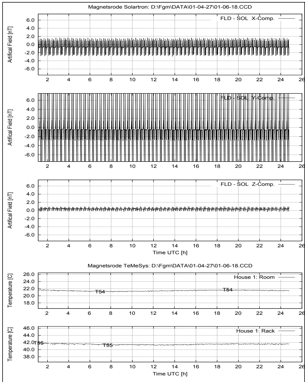
Figure 90: April 27, 2001: System Performance: FLD – SOL; Temperatures at House 1.
