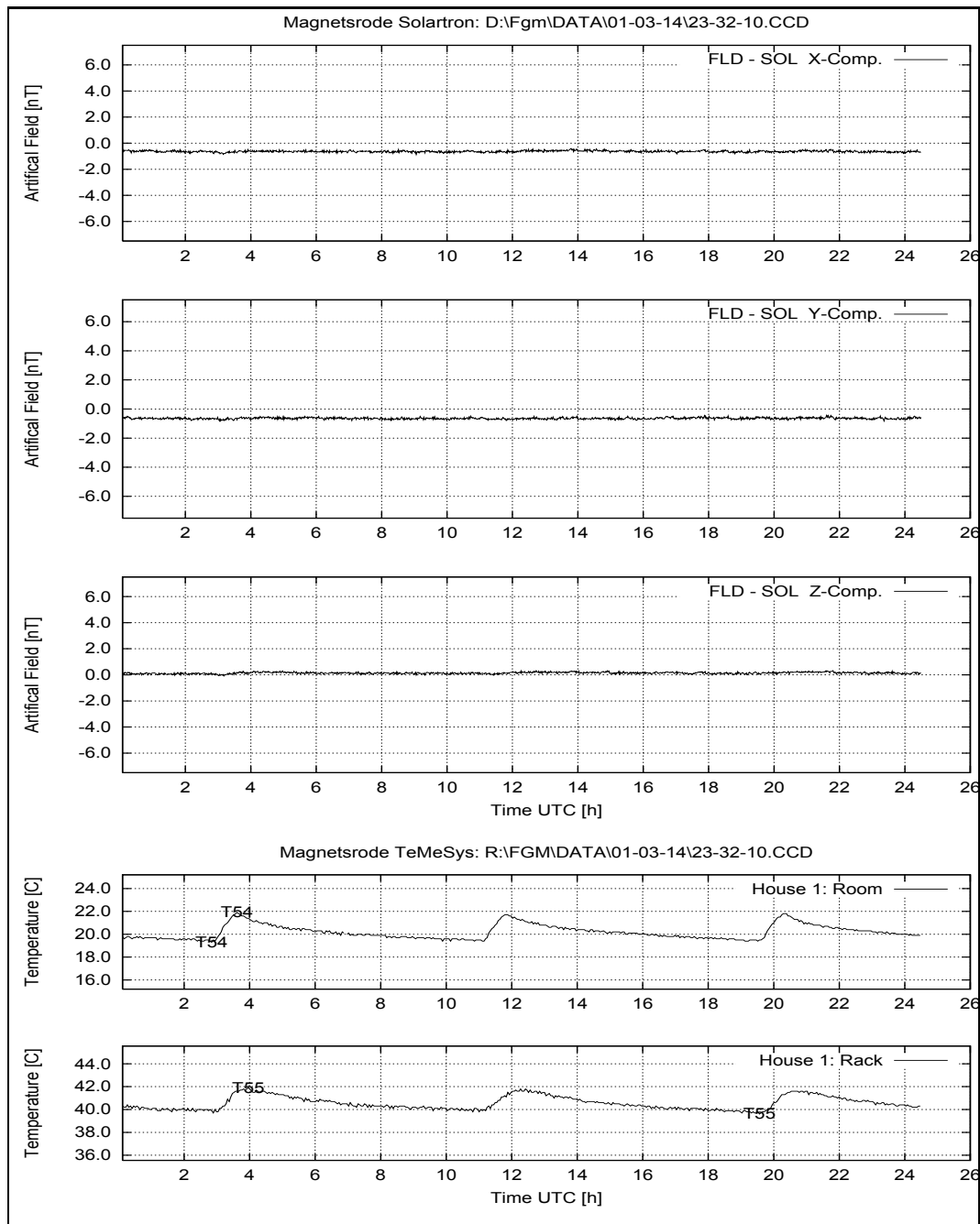
Figure 201: March 14, 2001: System Performance: FLD – SOL; Temperatures at House 1.
