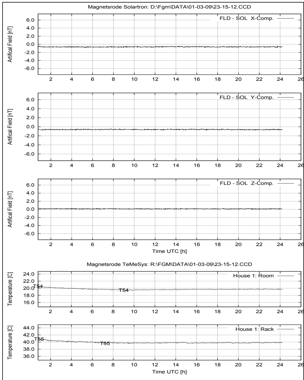
Figure 181: March 9, 2001: System Performance: FLD – SOL; Temperatures at House 1.
