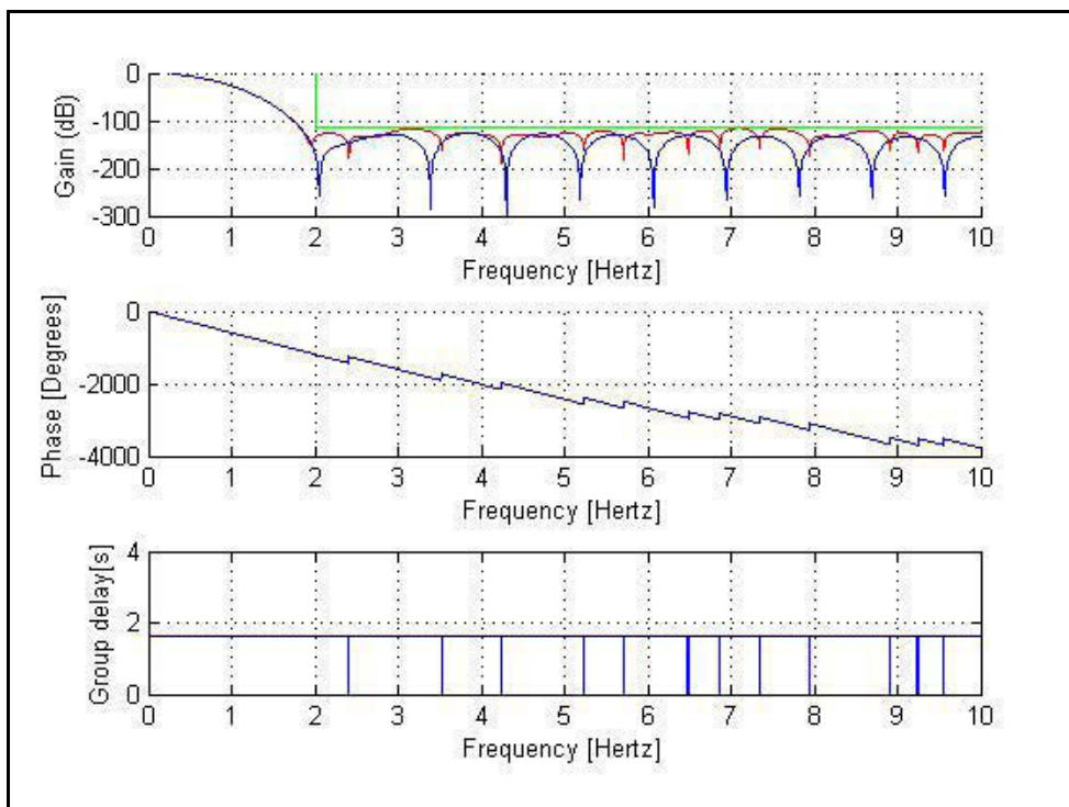
Amplitude, Phase Response and Group Delay of the Digital Filter for Filter-ID 1.
