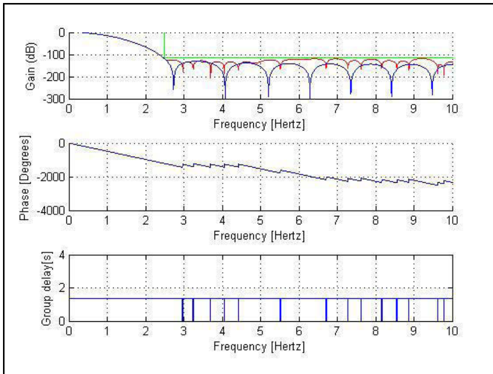
Amplitude, Phase Response and Group Delay of the Digital Filter for Filter-ID 2. Cutoff frequency = 2.5Hz, Decimation 4:1, Group delay = 1.35 s
