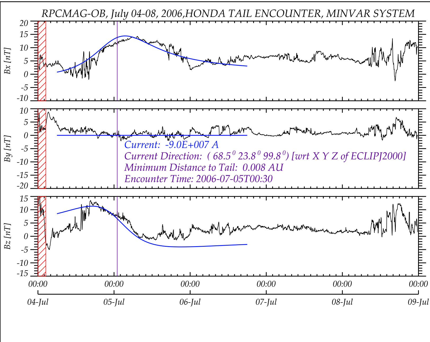
Figure 42: The observed magnetic field structure rotated to the Minimum Variance System
