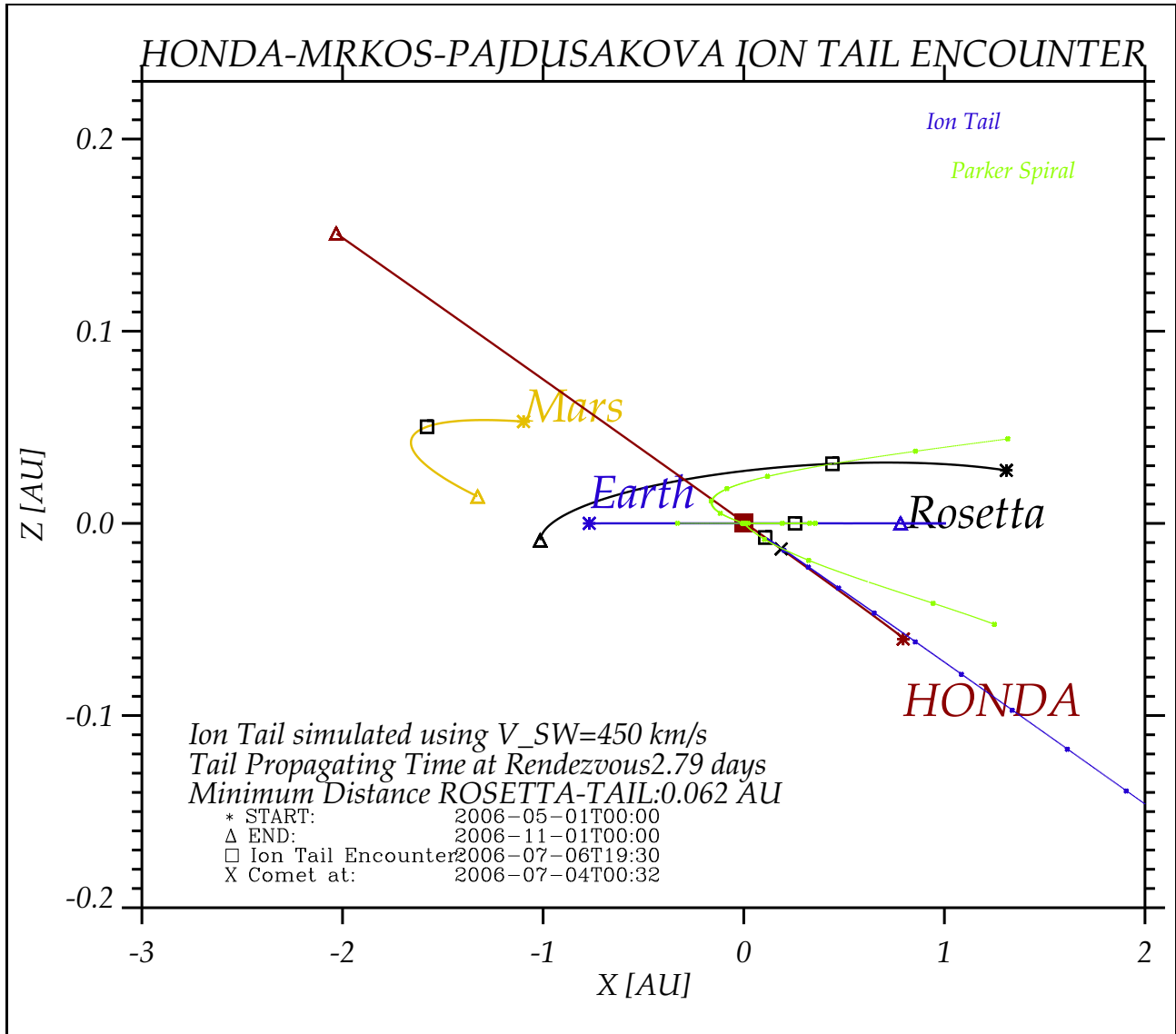
Figure 39: The geometrical encounter situation in the xz-plane (ECLIPJ2000)
