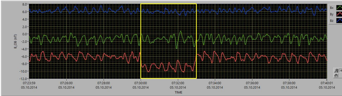
Figure 1: Example of a well resolved WOL disturbance recorded on 05.10.2014 during the PRL-phase with the OB sensor. The x-axis shows a 16-minute interval and the y-axis shows the magnetic field components in a total range of 20 nT. The yellow rectangle marks the duration of the disturbance. The WOL effects the magnetic field mainly in y-direction (red line) and during switch off the x-component shows a phase jump.
