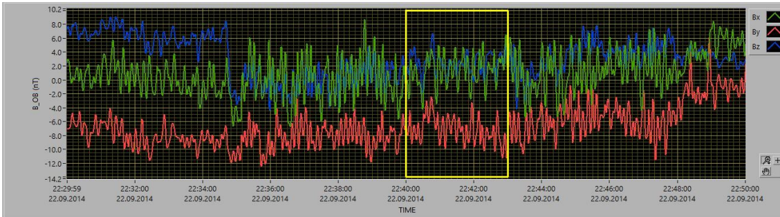
Figure 2: Example of a not visible WOL disturbance recorded on 22.09.2014 during the PRL-phase with the OB sensor. The x-axis shows a 20-minute interval and the y-axis shows the magnetic field components in a total range of 24 nT. The yellow rectangle marks the duration of the disturbance.
