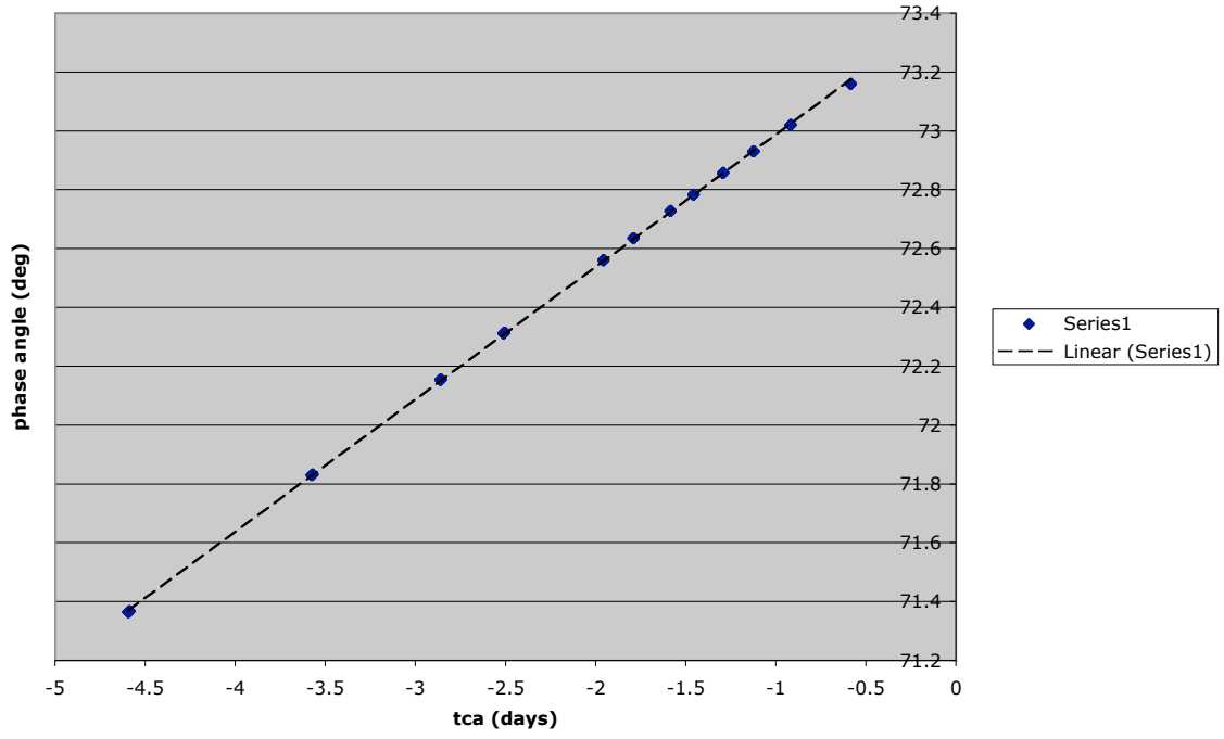
phase ange vs time from closest approach
